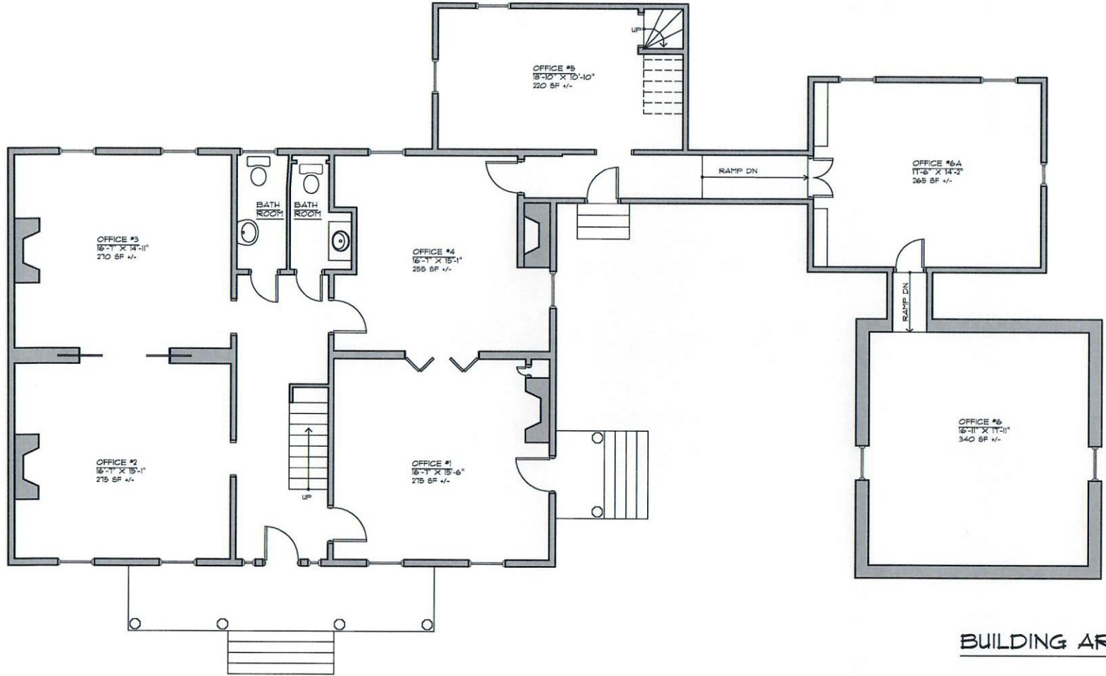
FIRST FLOOR PLAN SCALE 1/8" = 1'-0" 2,320 SF
